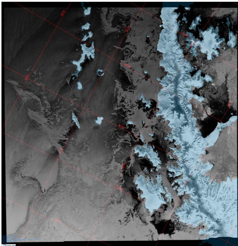
Sentinel-1 Satellite image of the sea ice around Anvers Island October 18, 2020
