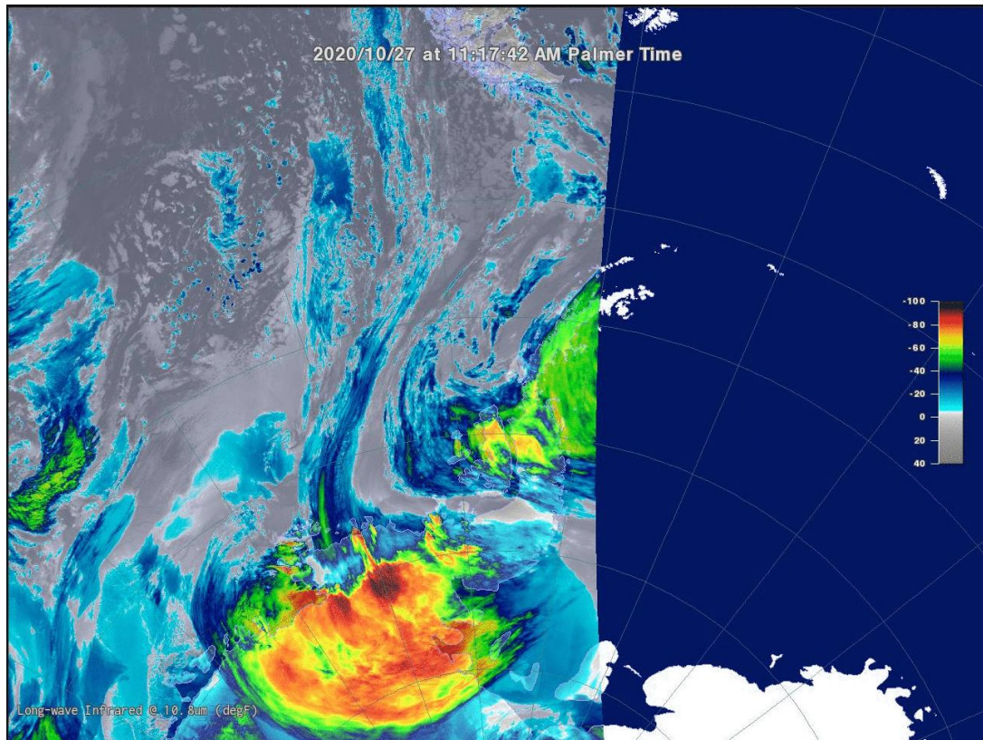
NOAA-18 satellite pass from October 27 th at 11:42 am local time
