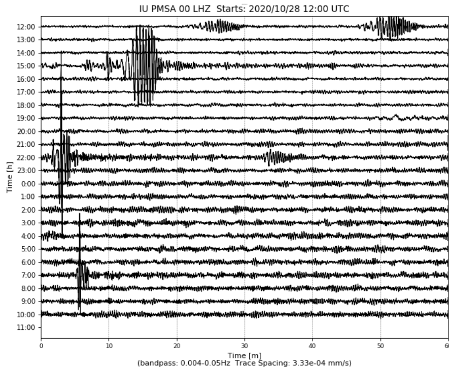
Heliplot of several earthquakes in the South Shetland Islands on October 28 th , 2020
